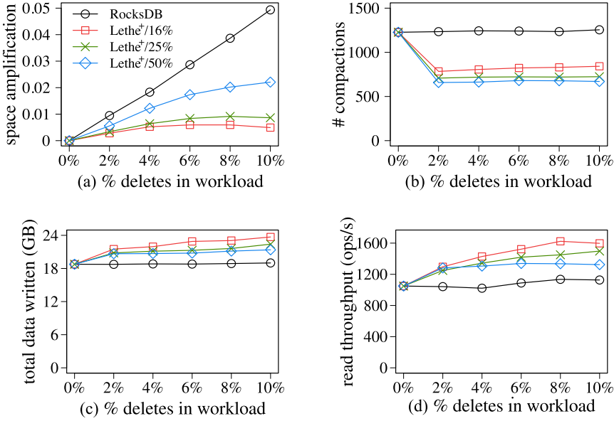
Fig. 7. Lethe+ reduces space amplification (a) and performs fewer larger compactions (b, c) to persist deletes timely, and in the process, by purging logically invalidated entries eagerly also improves read throughput (d).
